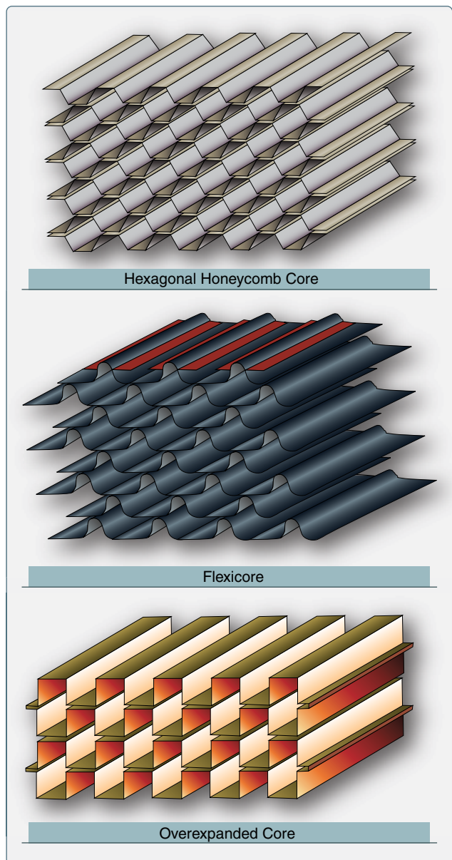
Figure 7-20. Honeycomb density.
