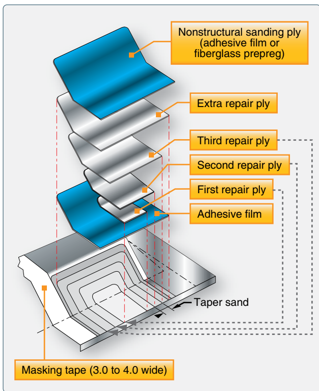
Figure 7-66. Trailing edge repair.
